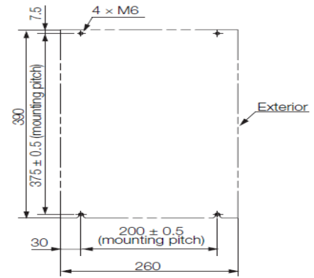
Mounting Hole Diagram Approx. Mass: 15.5 kg Unit: mm
