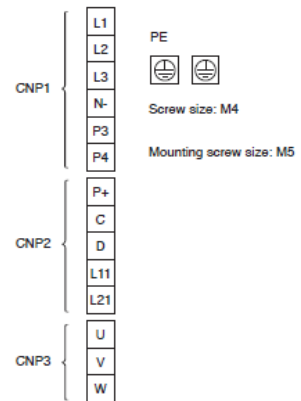
Terminal arrangement
